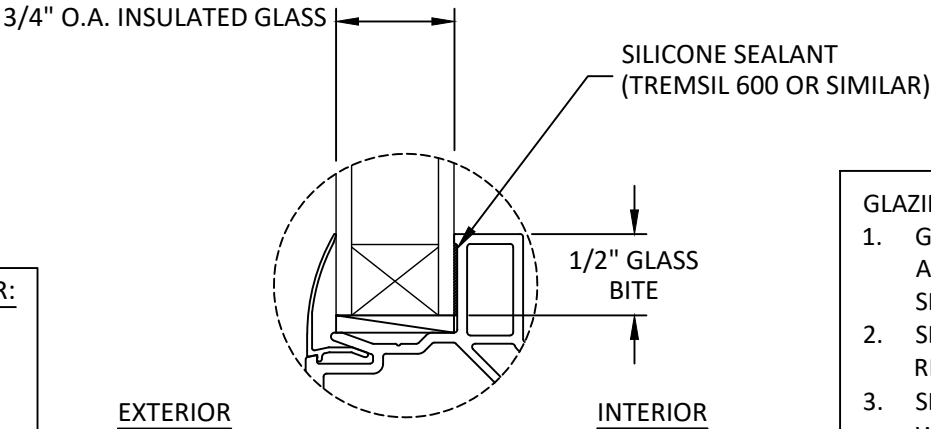
GLAZING DETAIL 1
