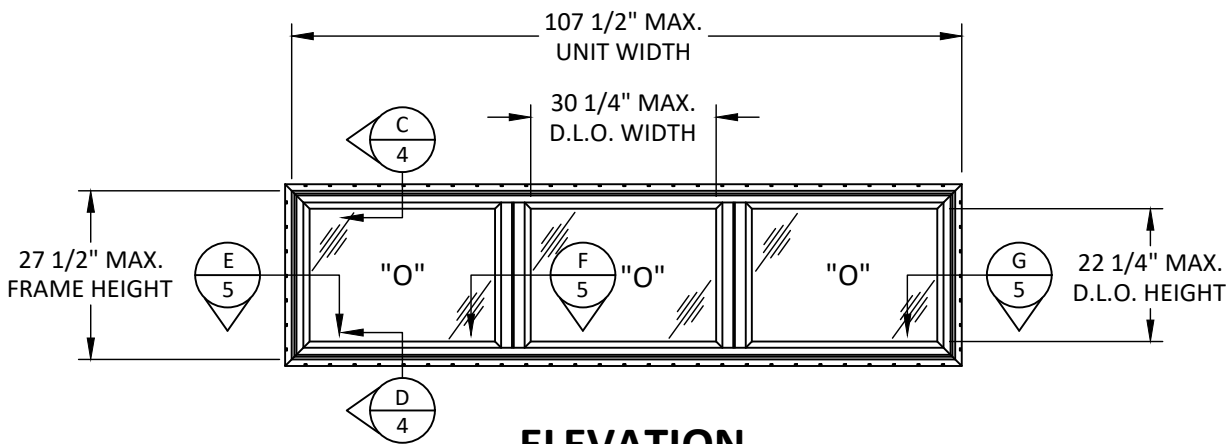
ELEVATION TRIPLE TRANSOM WINDOW DP50
