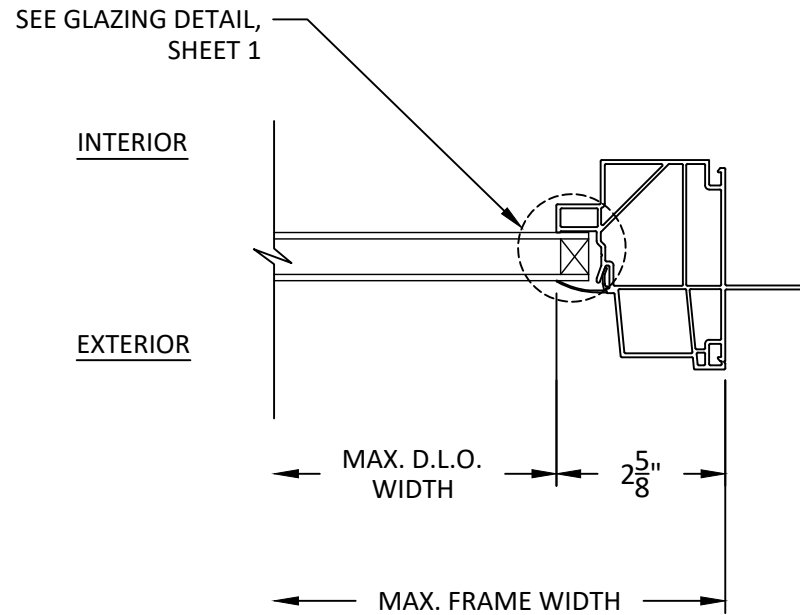
G5 HORIZONTAL SECTION FIXED & TRANSOM JAMB
