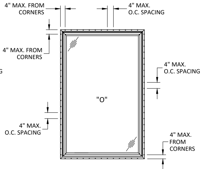
ANCHOR LAYOUT NAILING FIN
