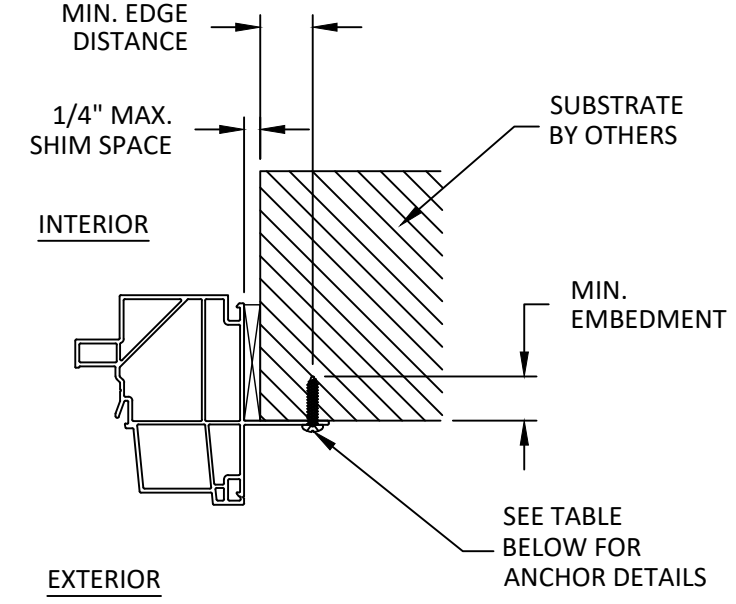
C 6 HORIZONTAL SECTION JAMB INSTALLATION
